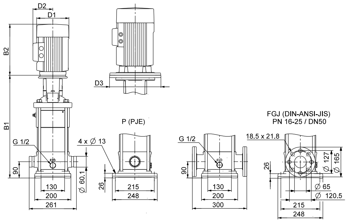
CRN 15, CRN 20
