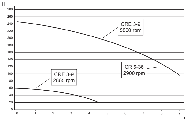
Comparison of performance: CRE 3-9 running at over-synchronous speed matching the performance of a CR 5-36 running at rated maximum speed
