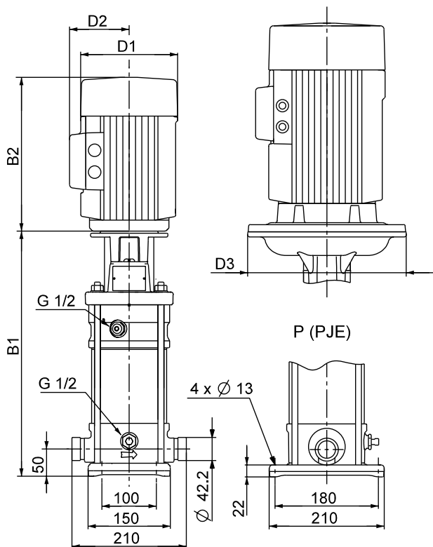
CRN 5
