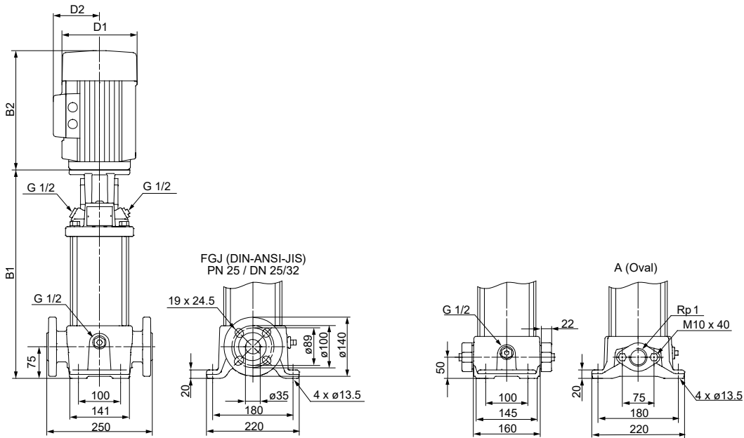
CR 1, CR 3
