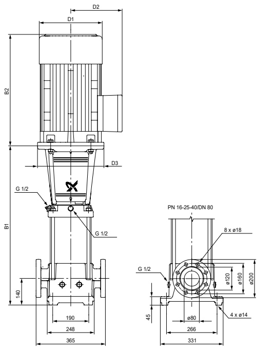
CR 45
