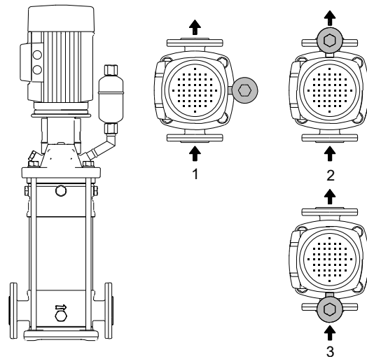
Vent positions on vertical CR 1s-64 pumps
