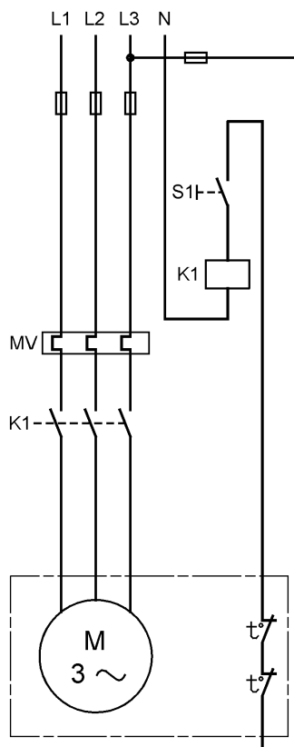
Typical circuit of a three-phase motor with built-in bimetallic thermal switches
