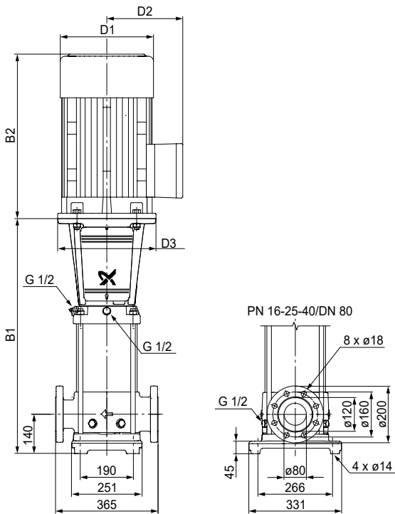
CRN 45
