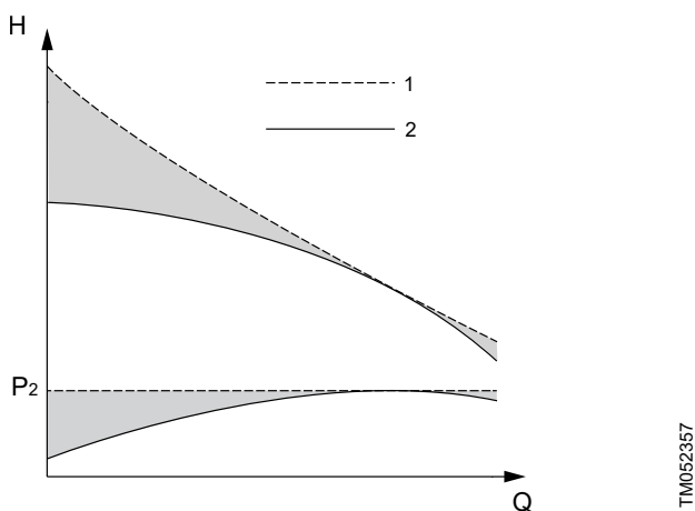
Curves of a standard E-pump and a pump operating at power limit
