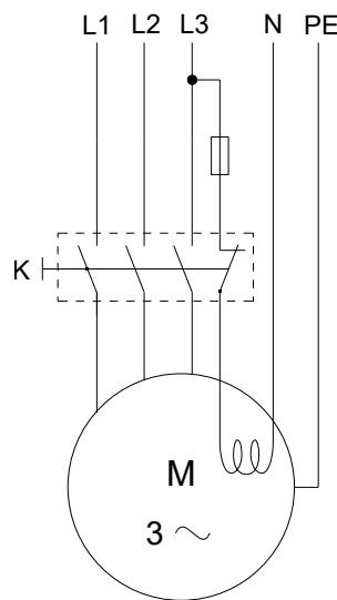
Three-phase motor with an anti-condensation heater
