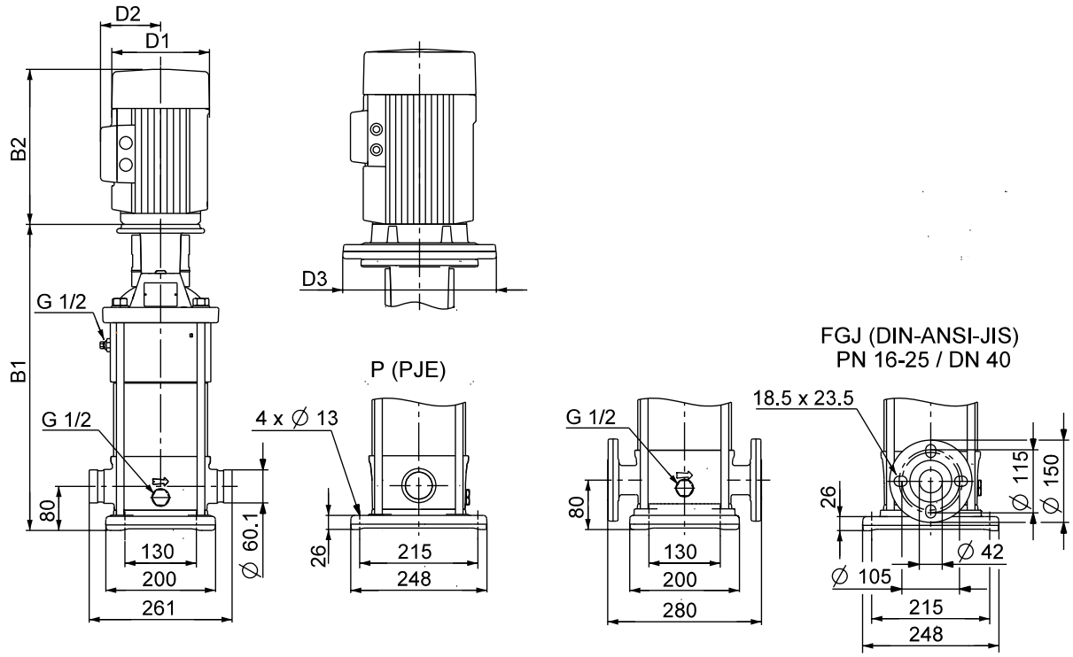
CRN 10
