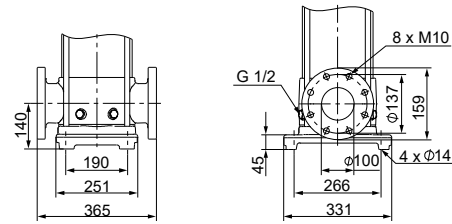
Collar connection for CRI, CRN 64
