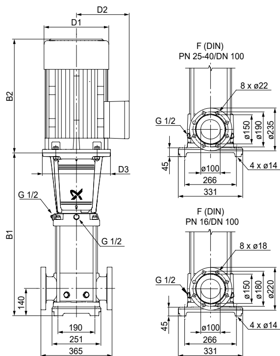
CRN 64
