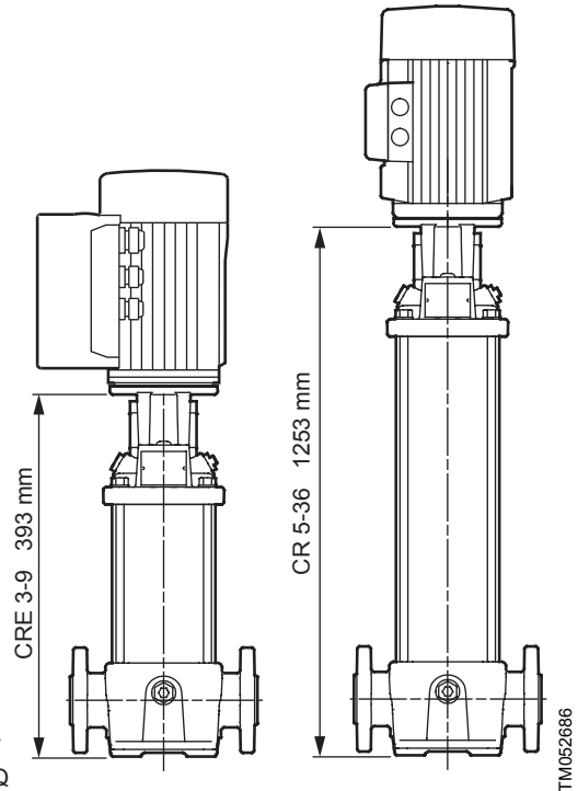
Comparison of performance: CRE 3-9 running at over-synchronous speed matching the performance of a CR 5-36 running at rated maximum speed
