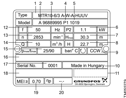
Example of a pump nameplate
