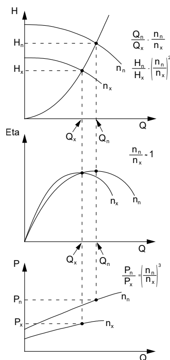
Affinity equations
