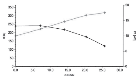
Measured values for tested pump
