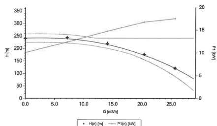
Measured values calculated to nominal speed n_{nom}
