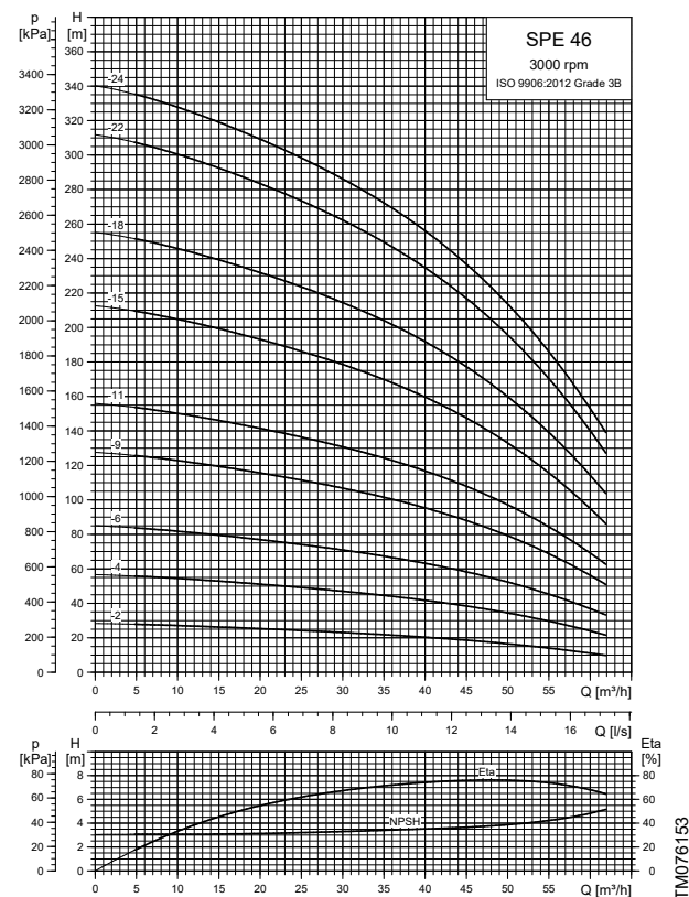
Example of an SPE pump's duty point
