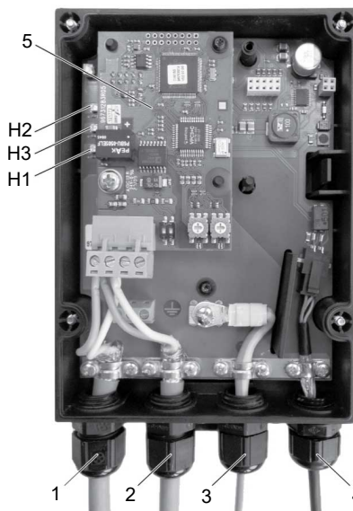
E-box overview
