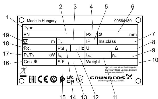
Nameplate
