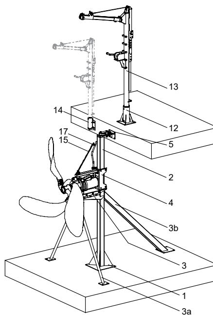
SFG installation
