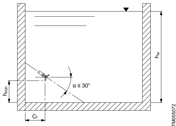
Mixer pointing downwards
