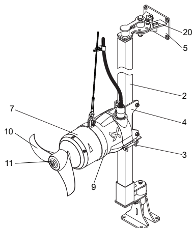
SMD mixer
