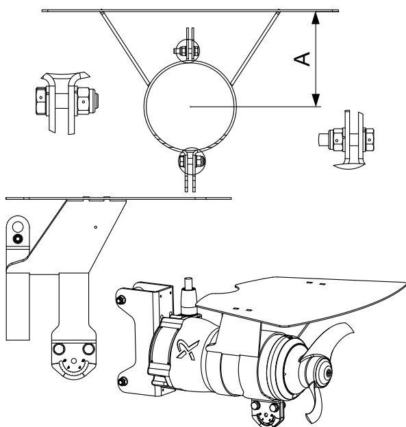
Vortex shield (SMD, T-version)
