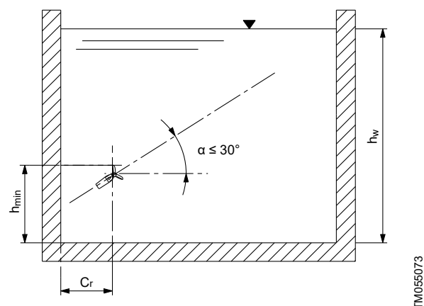
Mixer pointing upwards
