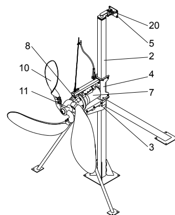
SFG flowmaker
