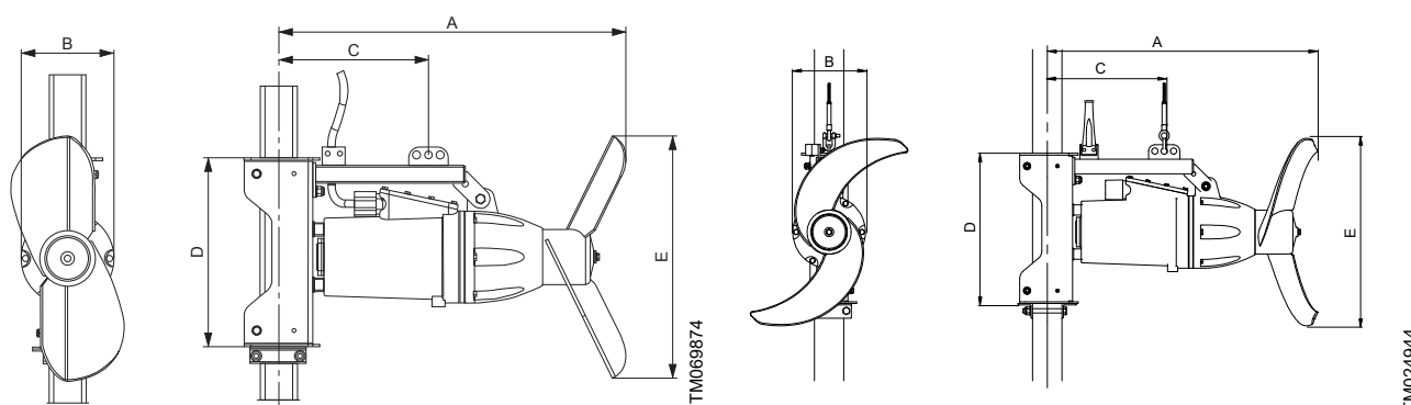
H - propeller design
