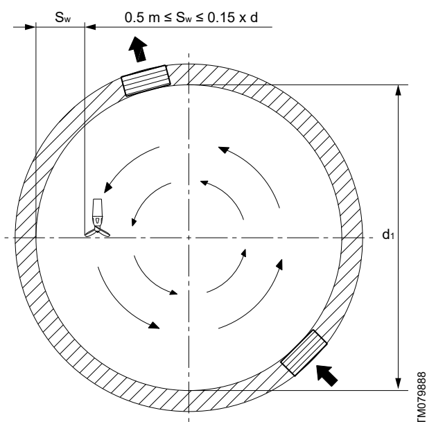
Vortex circulation of liquid
