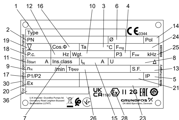
Nameplate of explosion-proof SMD mixers
