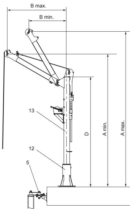
Crane
