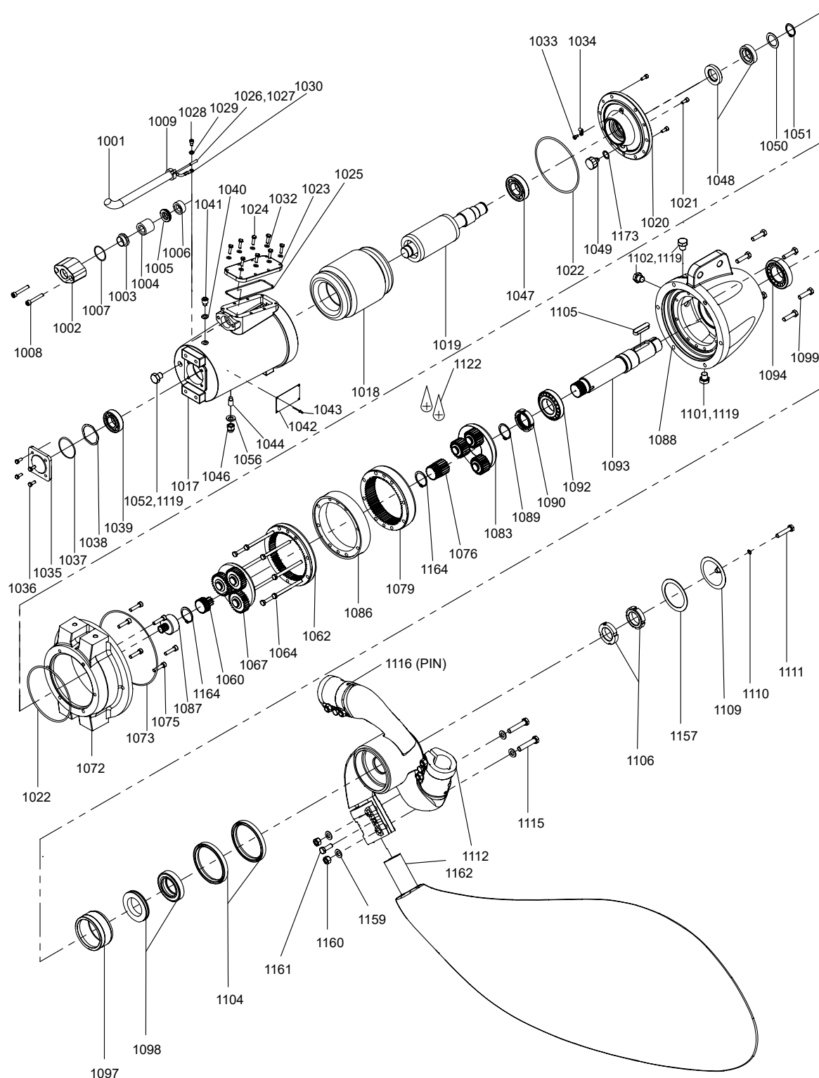
Exploded view, SFG.xx.180.xx and SFG.xx.230.xx
