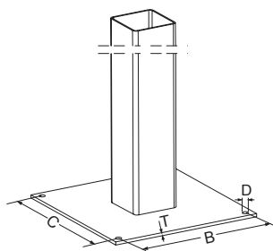
Bottom fixation plate - SFG.xx.130
