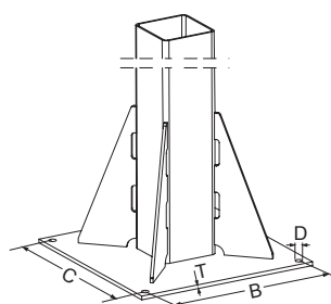
Bottom fixation plate - SFG.xx.180/230/260
