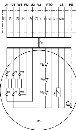
Three thermal switches (PTO)
