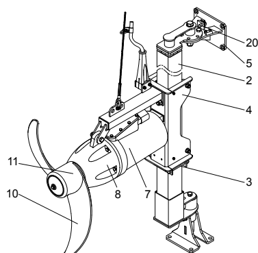
SMG mixer
