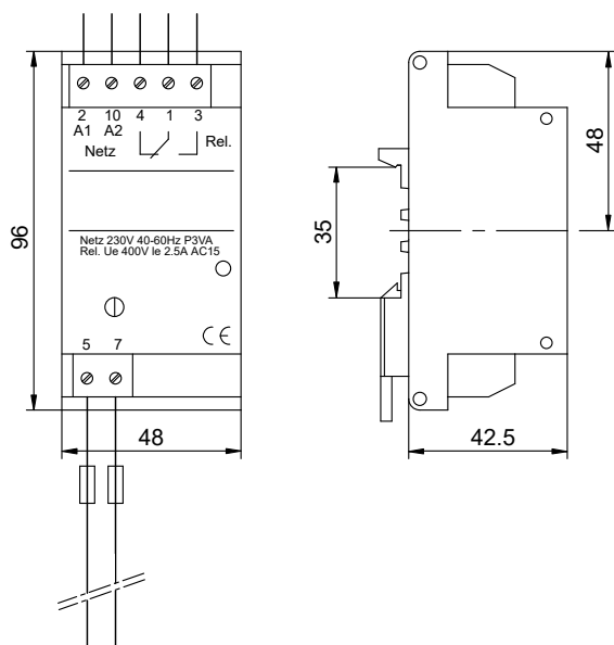
ALR-20/A-Ex relay
