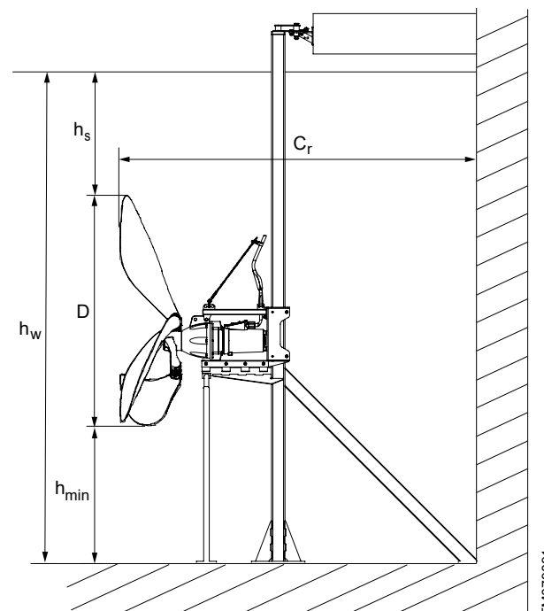
Schematic drawing of positioning of flowmakers
