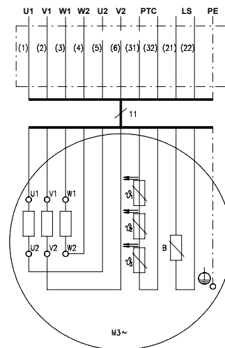
Three thermistors (PTC sensors)
