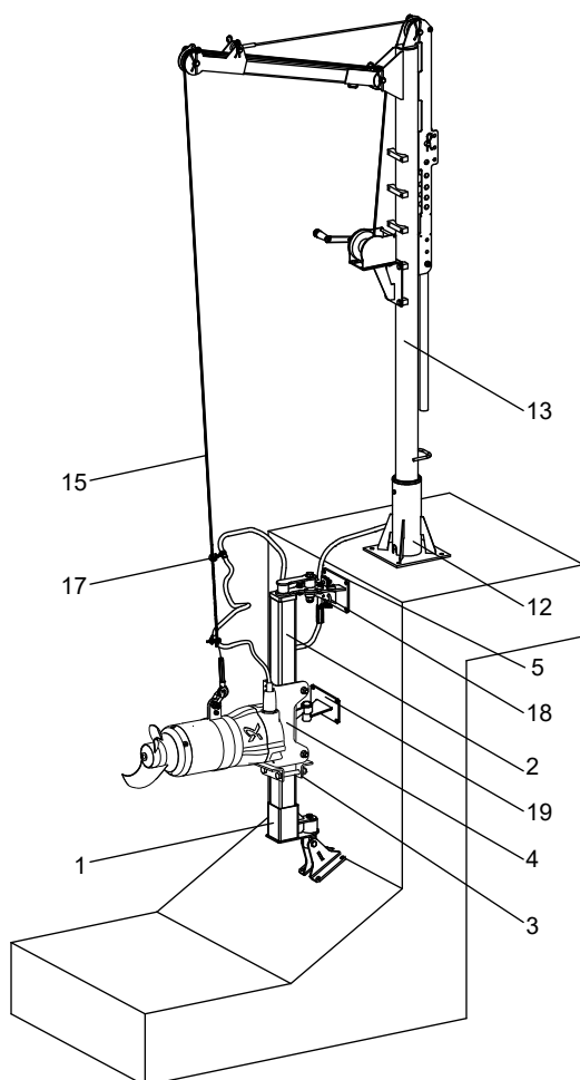
SMD mixer installed on a column profile
