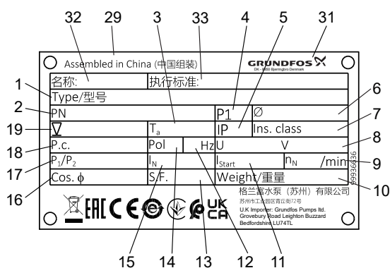
Nameplate for non-explosion proof products in China
