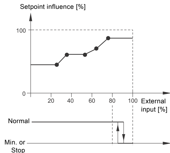
Fig. 42 Influence table with Stop at Max.
