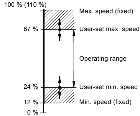
Fig. 34 Example of min. and max. settings
