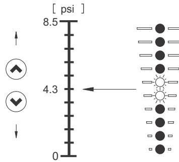
Fig. 15 Setpoint set to 4.3 psi (3 m), differential-pressure control
