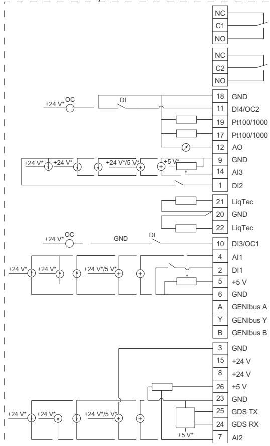
Fig. 9 Connection terminals, FM 300 (option)
