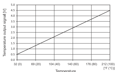
Fig. 163 Temperature response
