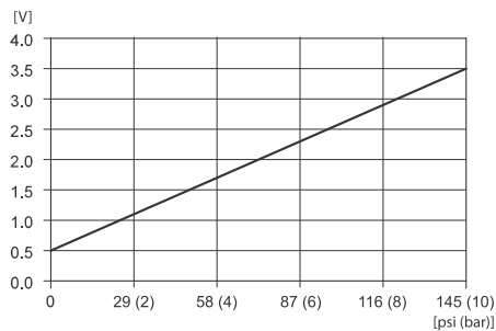
Fig. 130 Pressure response
