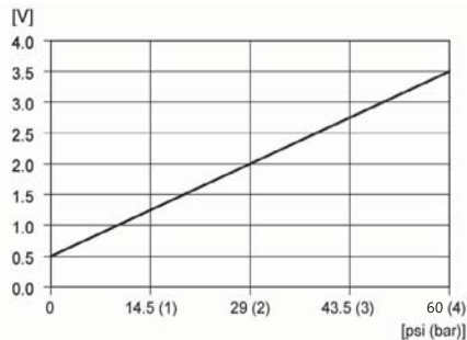
Fig. 122 Pressure response
