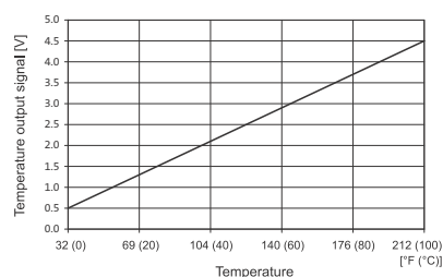
Fig. 138 Temperature response
