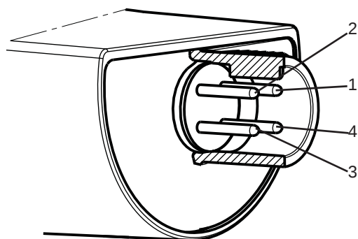
Fig. 42 Electrical connections
