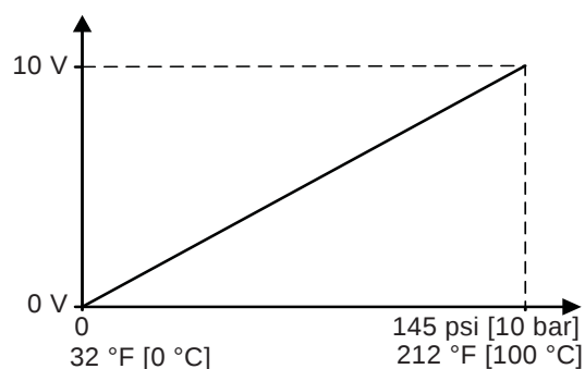
Fig. 70 Pressure and temperature response DPI+T
