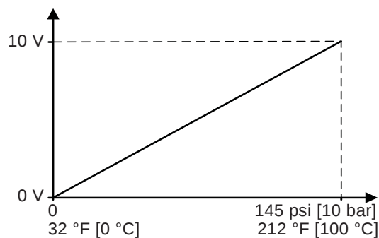
Fig. 32 Pressure and temperature response of RPI+T 0-10.0
