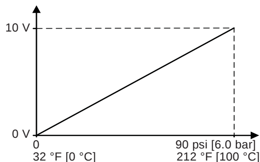
Fig. 28 Pressure and temperature response of RPI + T
