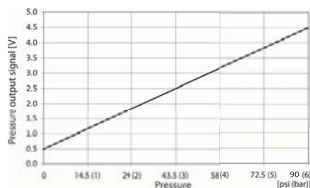
Fig. 162 Differential pressure response
