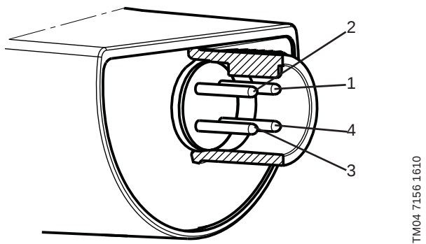
Fig. 4 Electrical connections
