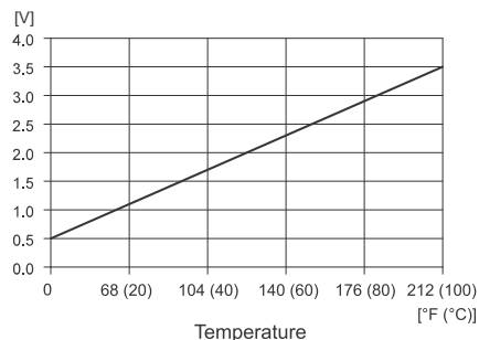
Fig. 123 Temperature response
