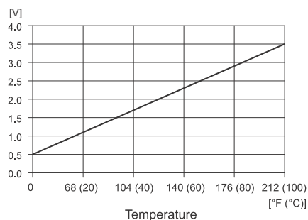
Fig. 107 Temperature response
