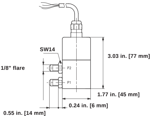
Fig. 84 Dimensions DPI transmitter
