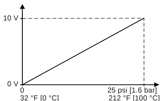
Fig. 54 Pressure and temperature response DPI+T
