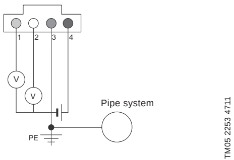
Fig. 133Electrical connections
