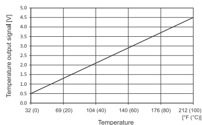
Fig. 153 Temperature response
