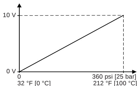
Fig. 46 Pressure and temperature response DPI +T
