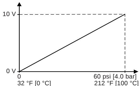
Fig. 24 Pressure and temperature response of RPI +T
