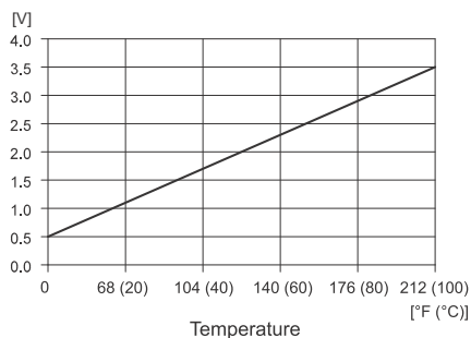
Fig. 131 Temperature response
