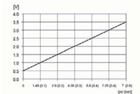
Fig. 106 Pressure response
