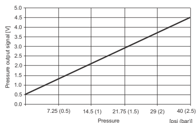
Fig. 152 Differential pressure response
