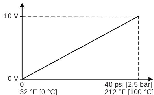
Fig. 20 Pressure and temperature response of RPI +T
