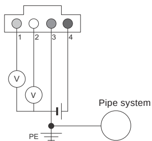
Fig. 102 Electrical connections
