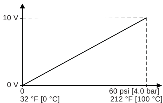
Fig. 62 Pressure and temperature response DPI+T
