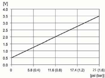
Fig. 114 Pressure response
