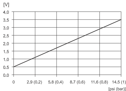
Fig. 110 Pressure response
