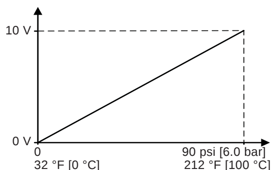
Fig. 66 Pressure and temperature response DPI+T
