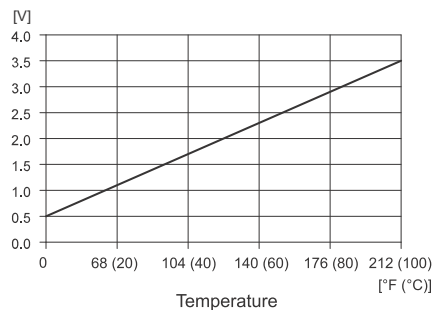
Fig. 115 Temperature response
