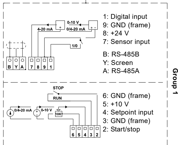
Fig. 14 Connection terminals - TPE, NKE, NKGE and NBE, NBGE, MTBE
