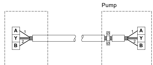
Fig. 18 Connection with screened 2-core cable
