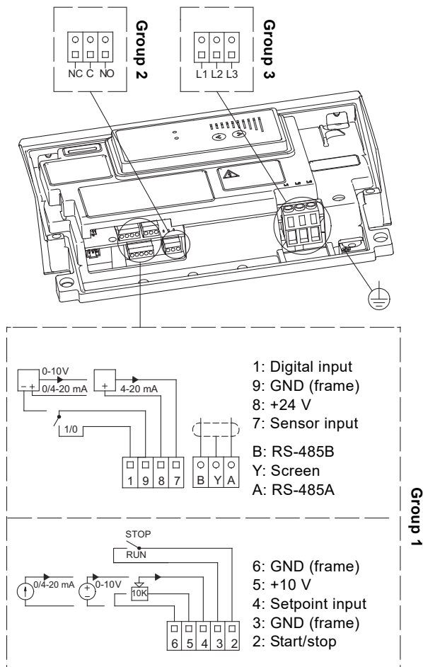
Fig. 8 Connection terminals - TPE, NKE, NKGE and NBE, NBGE, MTBE
