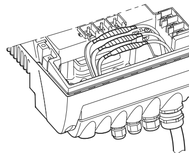
Fig. 44 Insulated conductors
