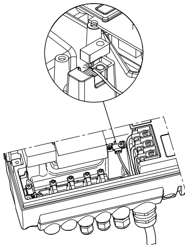
Fig. 11 Connection of a single protective earth conductor using one of the conductors of a 4-core mains cable (with cross-sectional area of min. 10 mm 2 )
