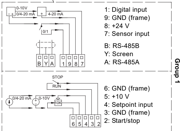
Fig. 5 Connection terminals - TPED
