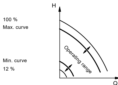
Fig. 33 Setting of the min. and max. curves in % of maximum performance
