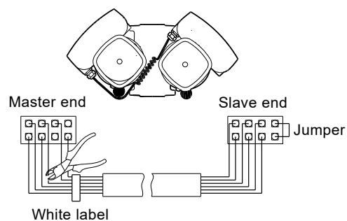
Fig. 22 Elimination of alternating operation and standby operation
