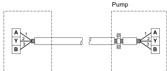
Fig. 17 Connection with screened 3-core cable
