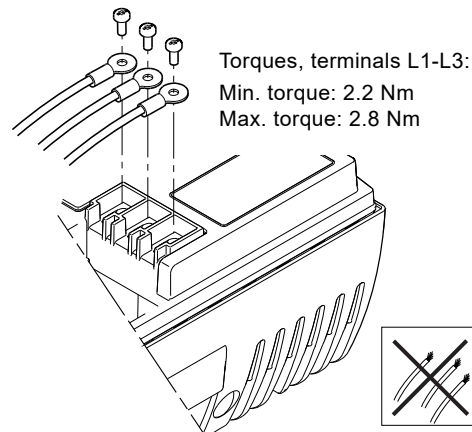
Fig. 13 Mains connection
