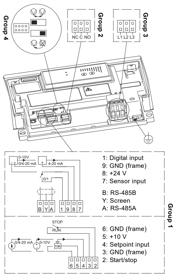
Fig. 9 Connection terminals - TPED
