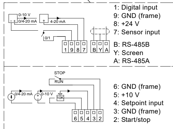
Fig. 4 Connection terminals - TPE, NKE, NKGE and NBE, NBGE, MTBE
