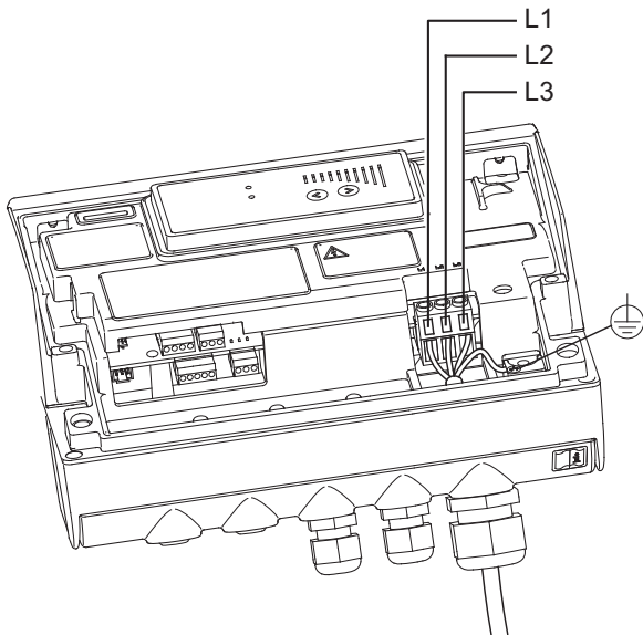
Fig. 7 Mains connection
